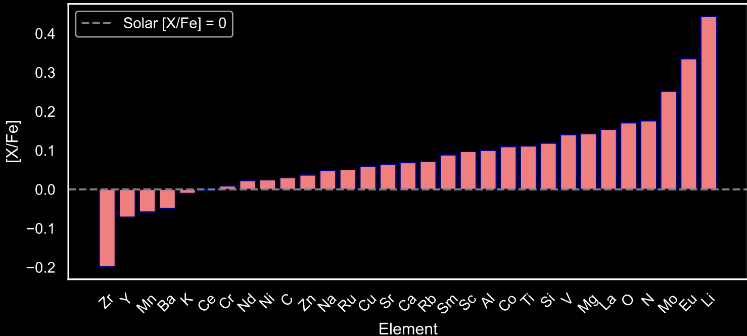
Abundance Pattern for GALAH Star Field [24] (N=274)
