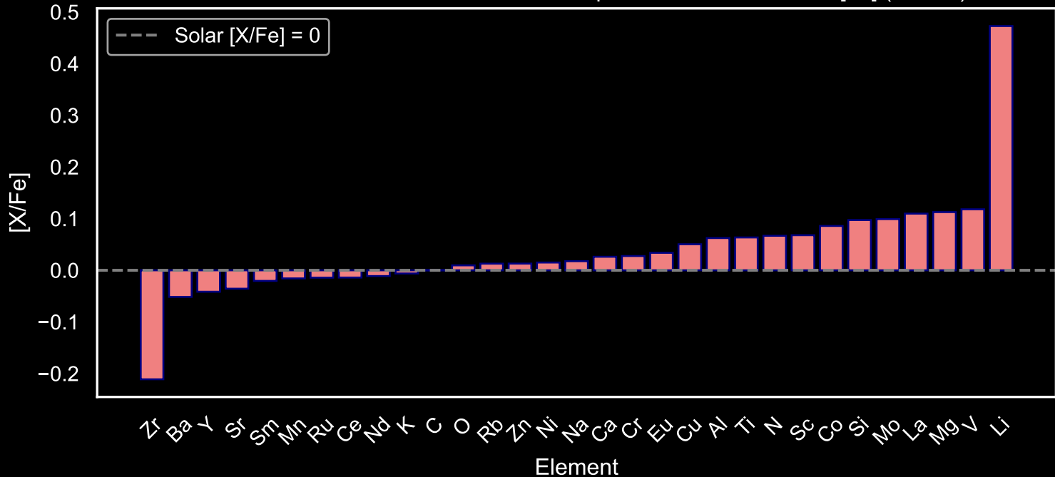
Abundance Pattern for GALAH Main Sequence Stars: Star Field [24] (N=128)
