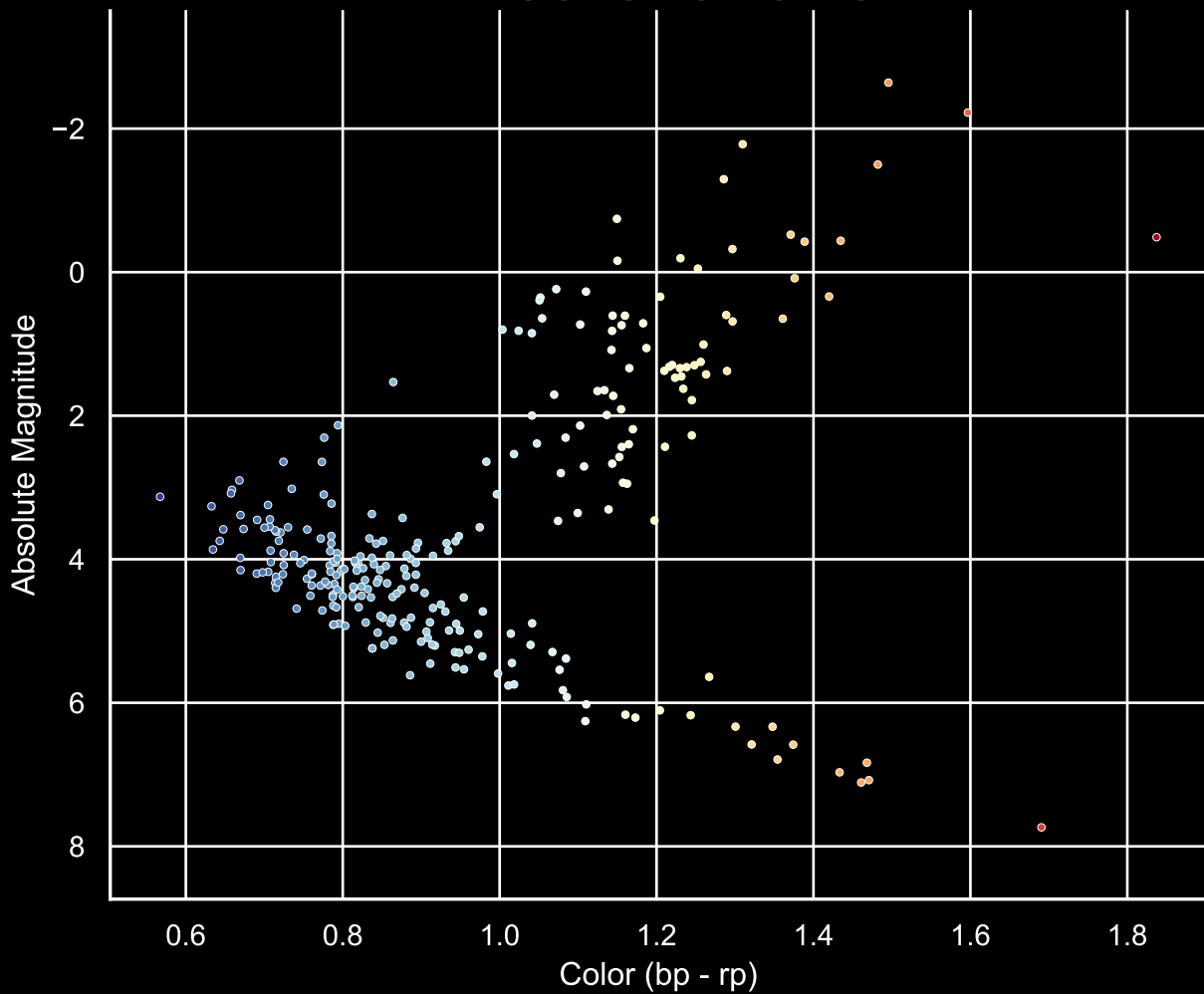
GALAH Hertzsprung-Russel Diagram Field [24] Ra [325.1] Dec [-52.69]
