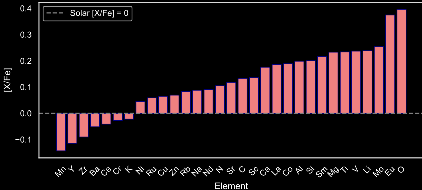
Abundance Pattern for GALAH Red Giants: Star Field [24] (N=75)
