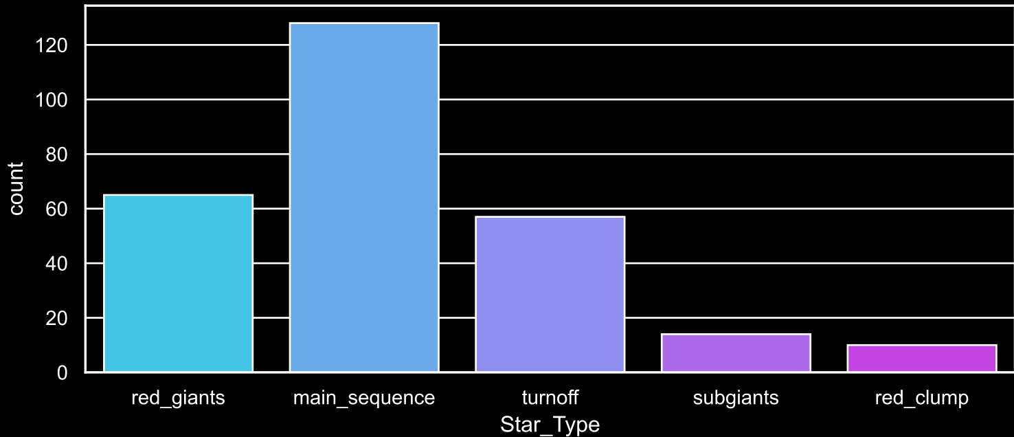
Field [24] Count plot of Star Type
